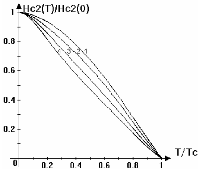
Fig.1. The temperature dependence H_{c2}(T)/H_{c2}(0) at \lambda_{11} = 0,2 , \lambda_{12} = 0,3 and values v_1/v_2 = 1, 2, 3 and 4 (curves 1-4 correspondingly)
